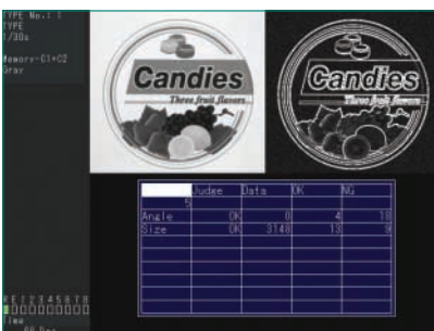
Simultaneous image display from two cameras (This shows an image processed with gray scale and binary differentiation.)
